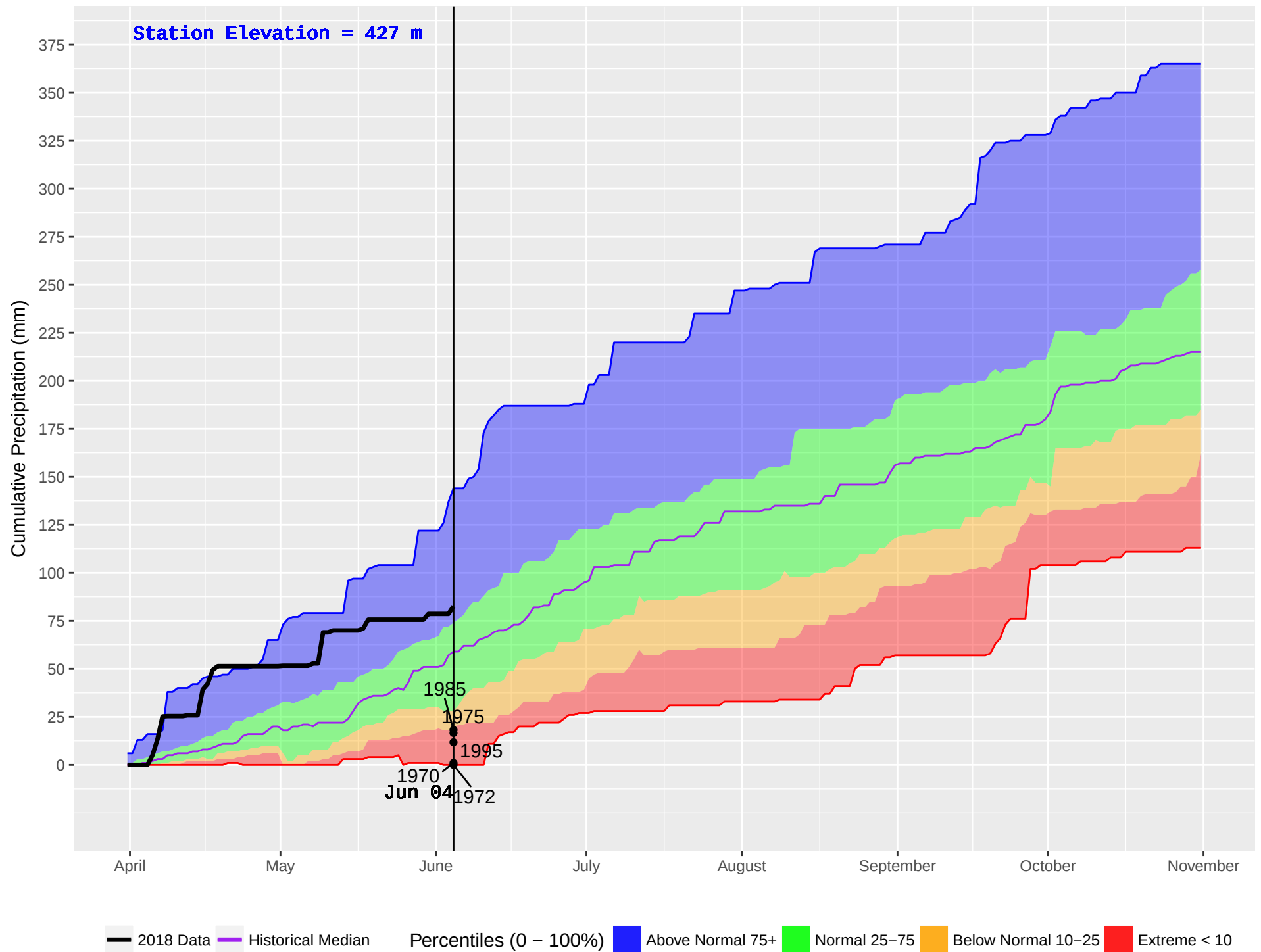
PENTICTON RS (328) : Historical (1970–2016) and Current (2018) Noon Cumulative Precipitation
