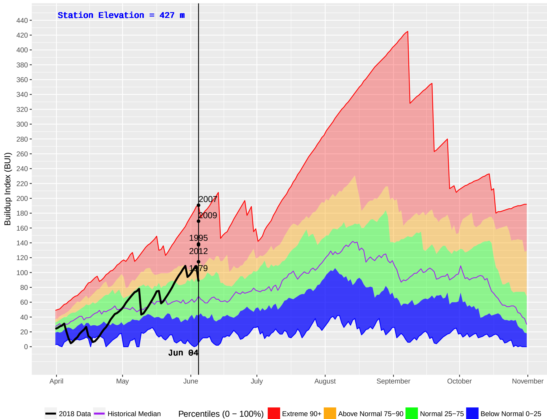
PENTICTON RS (328) : Historical (1970–2016) and Current (2018) Noon Buildup Index (BUI)
