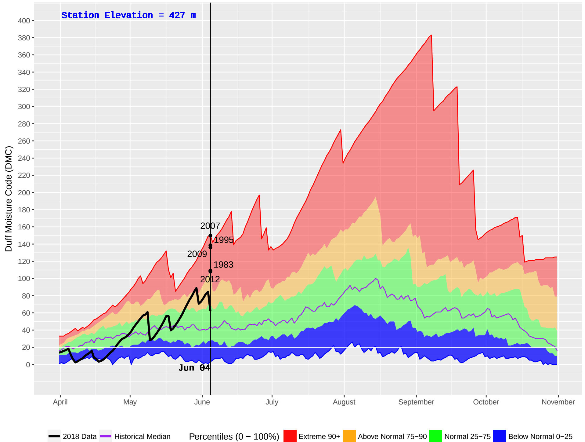
PENTICTON RS (328) : Historical (1970–2016) and Current (2018) Noon Duff Moisture Code (DMC)
